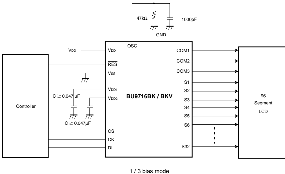
1 / 3 bias mode
