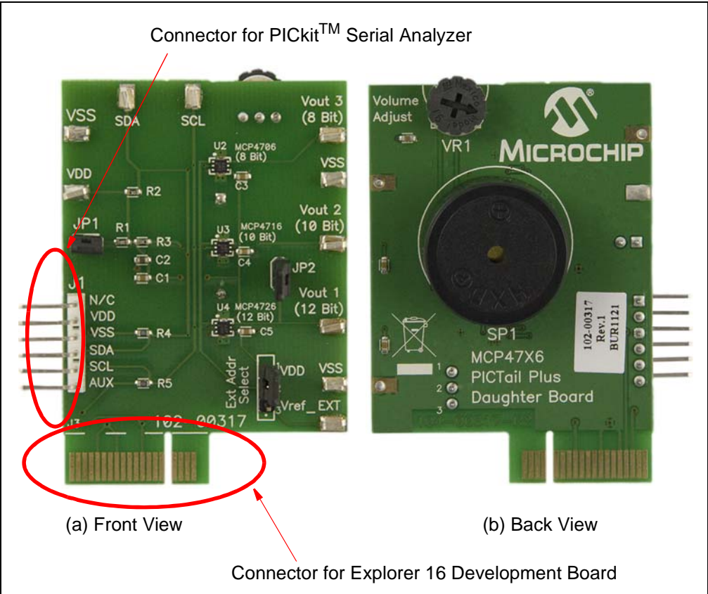
FIGURE 1-1: Front and Back Views of the MCP47X6 PICtail™ Plus Daughter Board.
